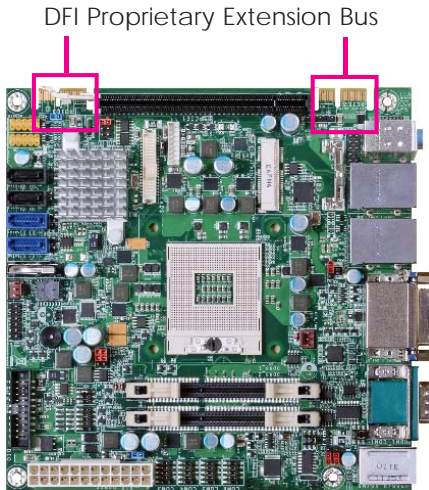
Motherboard
