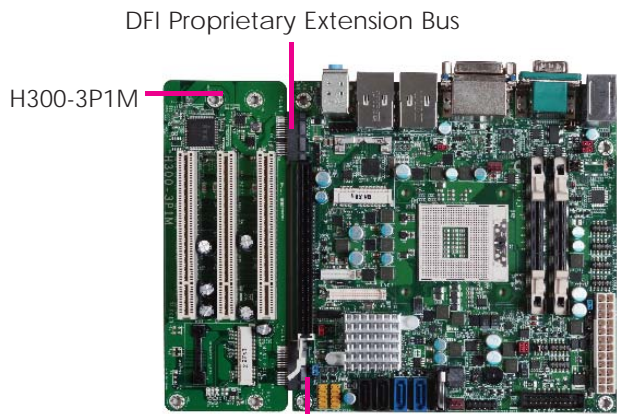
H300-3P1M Connected to the Motherboard
