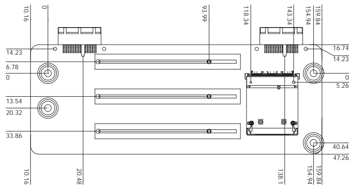
Mechanical Diagram
