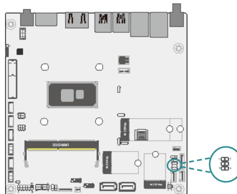
VCC Panel Power Select (DPJP3)
