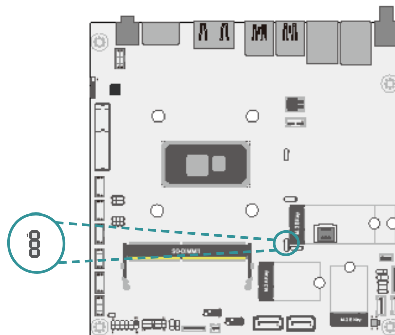
USB3-A/M.2 B-KEY (PBJP3)
