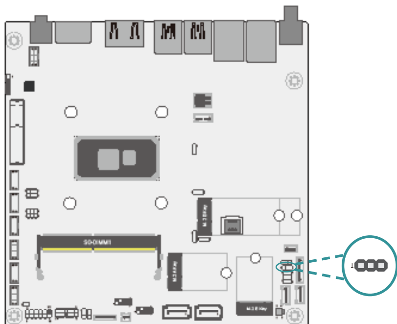
Inverter Panel Power Select (DPJP4)
