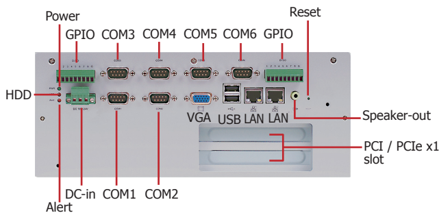
EC220-LR6G60 Rear View
