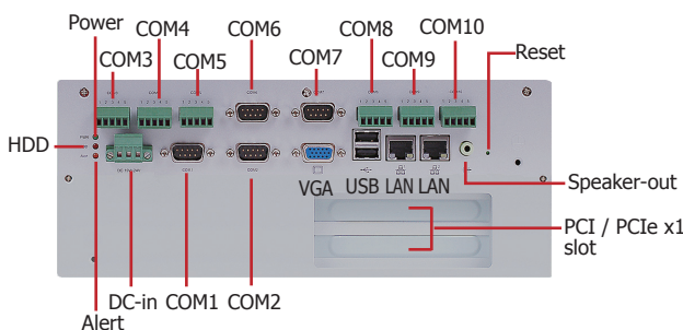
EC220-LRA060 Rear View
