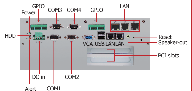
EC220-LR4G65 Rear View
