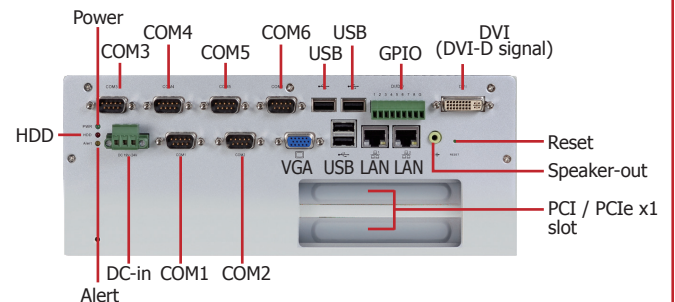
EC220/EC221-LRT6881 Rear View
