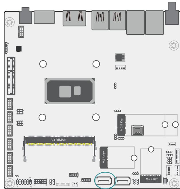
SATA0 (J4)
