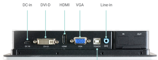
USB Type B port
