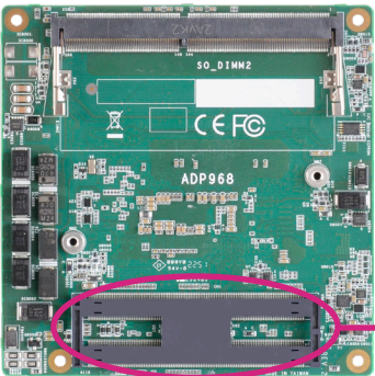
COM Express connector on ADP968
