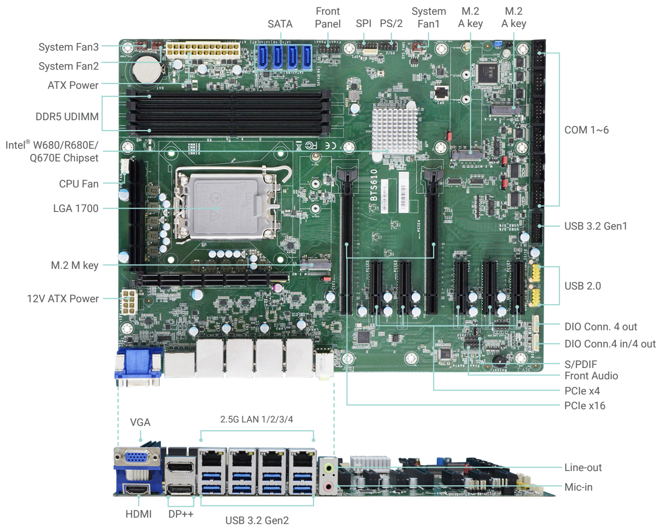
Top View (BTS610-W680/R680E)
