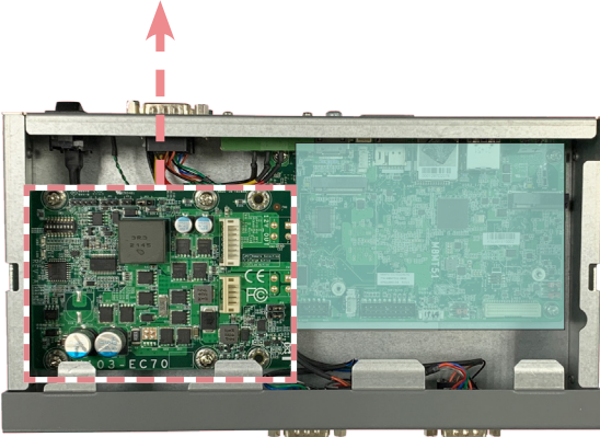
Power Board
