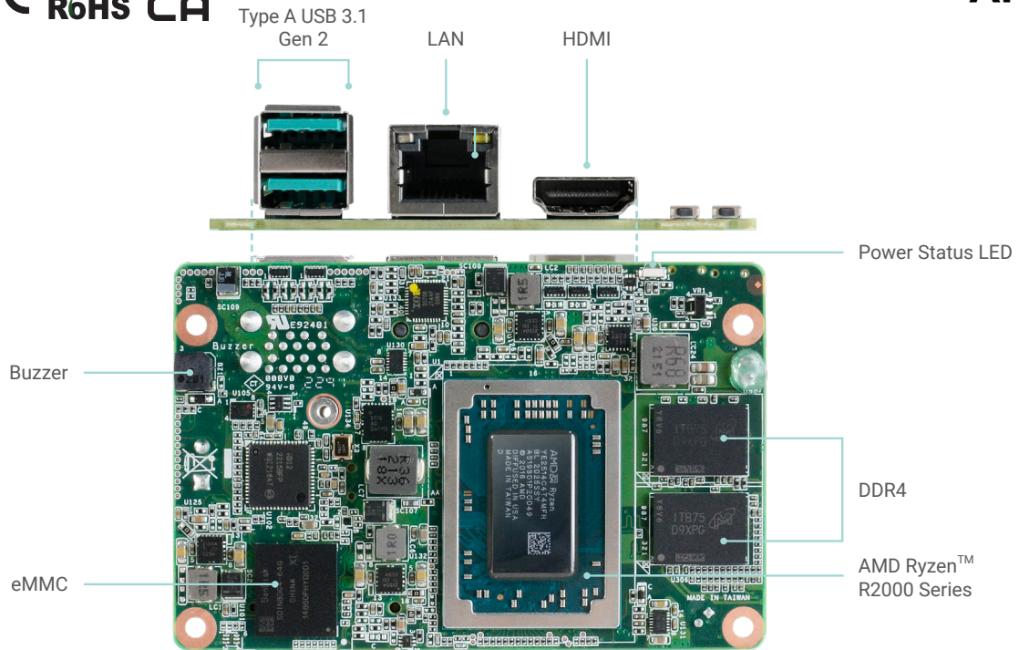
Bottom View
